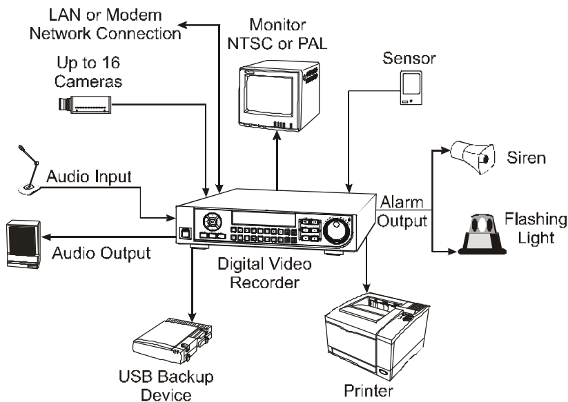
Figure 1 — Typical DVR installation.
