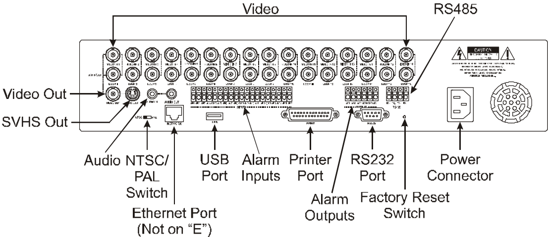
Figure 2 — 16-Channel DVR rear panel. (Others are similar.)
