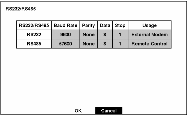
Figure 57 — RS232/RS485 setup screen.
